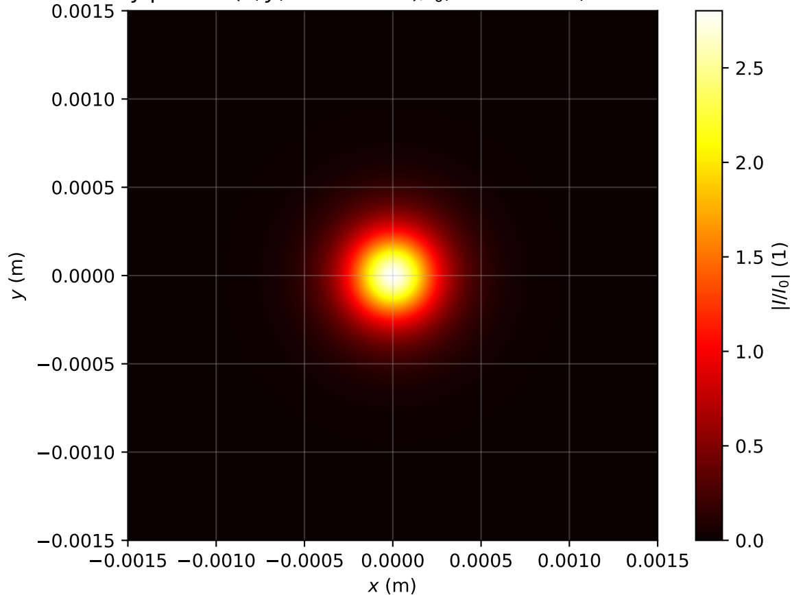
Intensity profile I(x, y, z = 3.264m)/I_0 , Pin=1.0Pcr, artificial time
